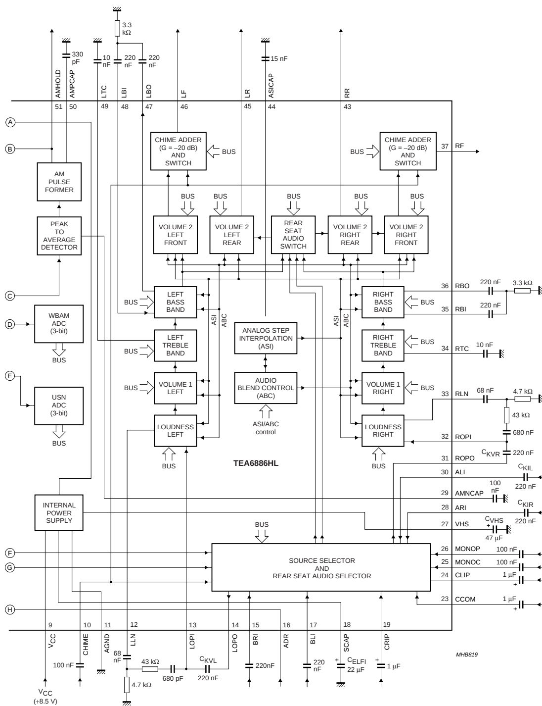
Fig.2 Block diagram (continued from Fig.1).
